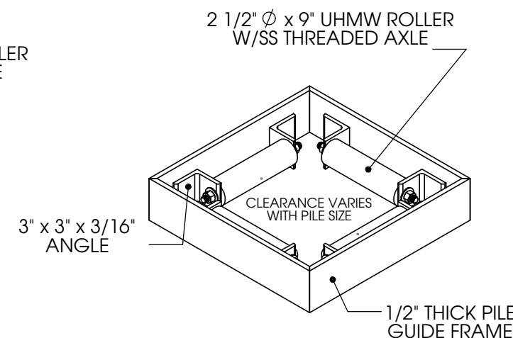
4-ROLLER INTERNAL PILE GUIDE
