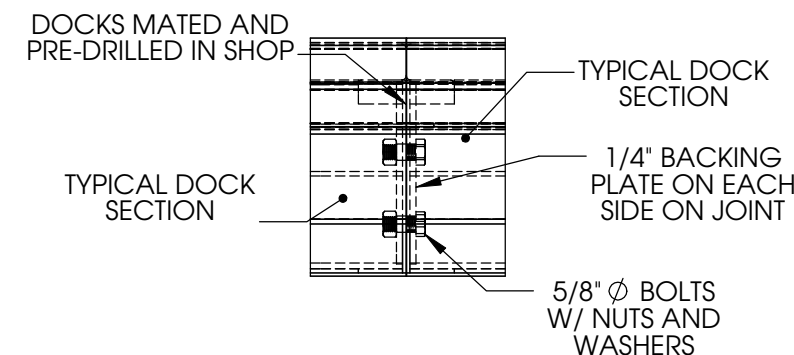
REINFORCED BOLTED DOCK CONNECTION
