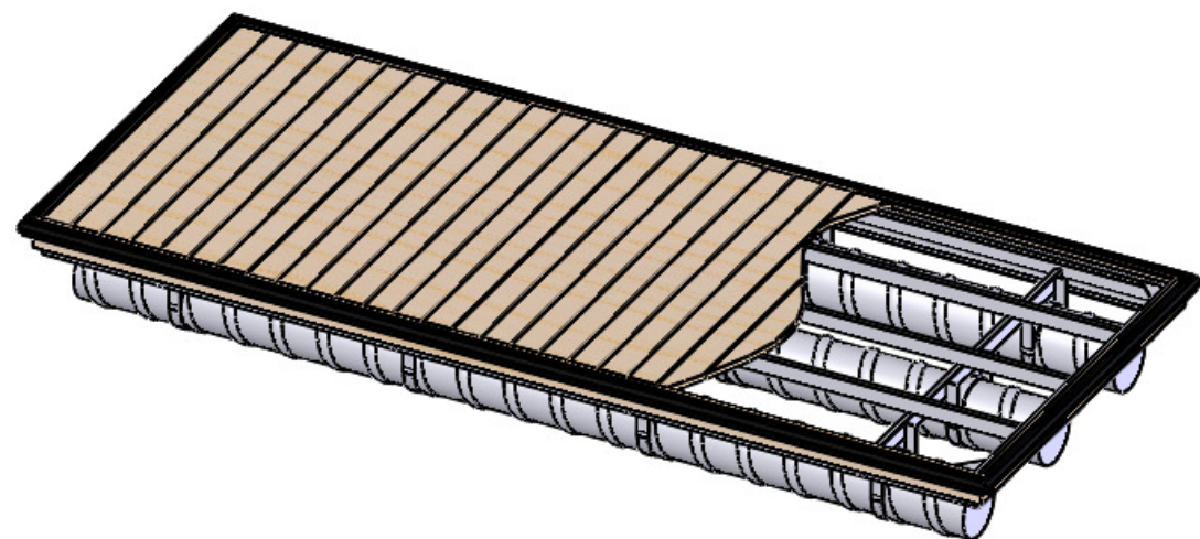
ISOMETRIC VIEW OF TOP DECKED PONTOON FLOATING DOCK
