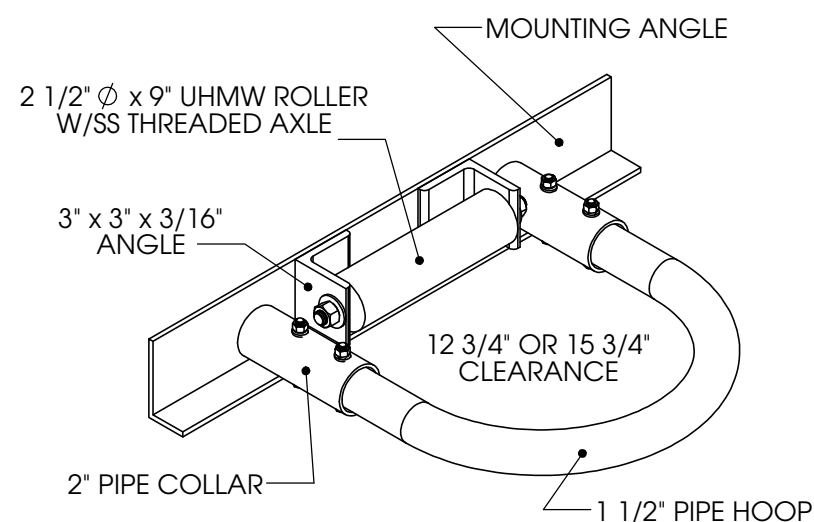
1-ROLLER EXTERNAL PILE GUIDE
