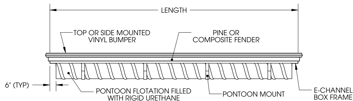
ELEVATION VIEW OF TOP DECKED PONTOON FLOATING DOCK
