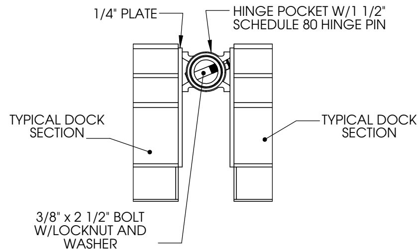
HINGED DOCK CONNECTION
