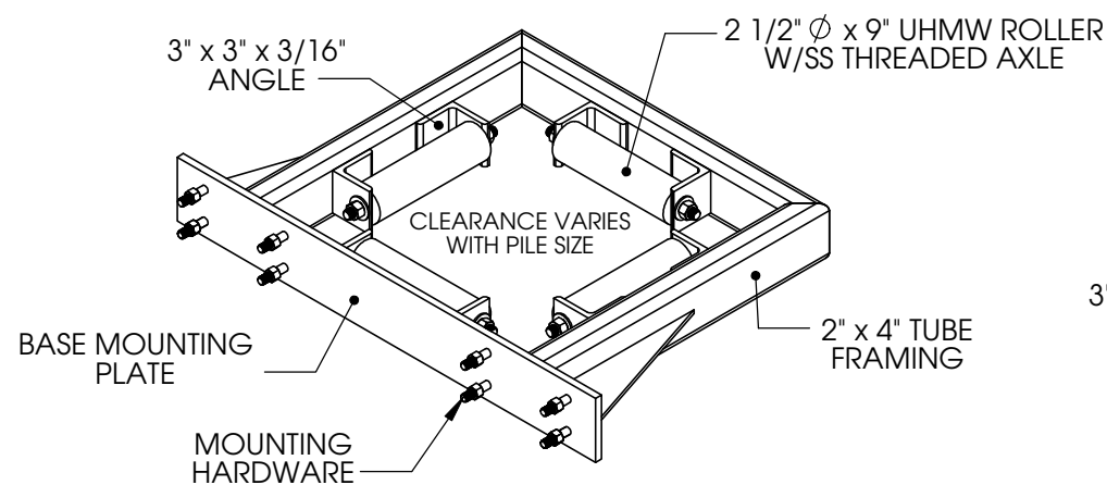
4-ROLLER EXTERNAL PILE GUIDE
