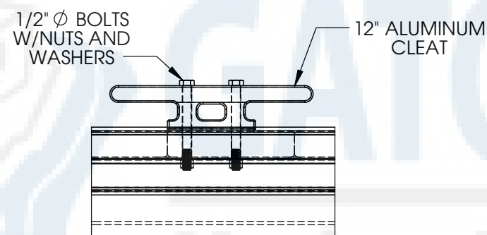
CLEAT DETAIL
