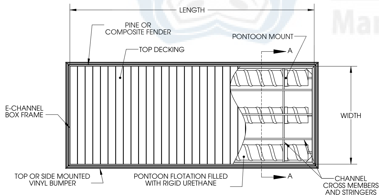
PLAN VIEW OF TOP DECKED PONTOON FLOATING DOCK
